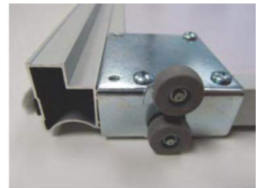
CODE SDS008 Sliding Door Wheel Set 4 Pieces (Sold 2 x Top + 2 x Bottom) See Below
